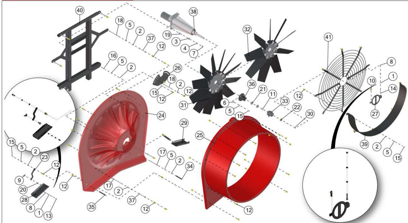
TURBINA Ø850mm
