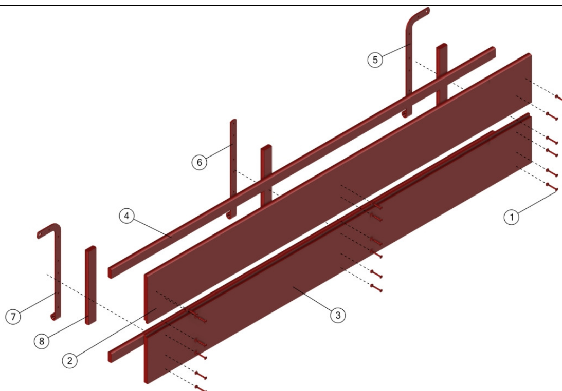
TAMPA LATERAL – CB-2
