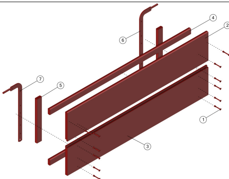
TAMPA TRASEIRA – CB-2
