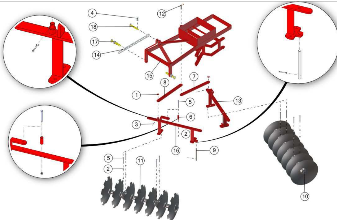
GRADE DE DISCOS – GVV/GVA 12x18" / 14x18"
